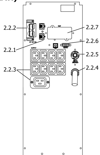
SXL-1500A~3000A LCD
